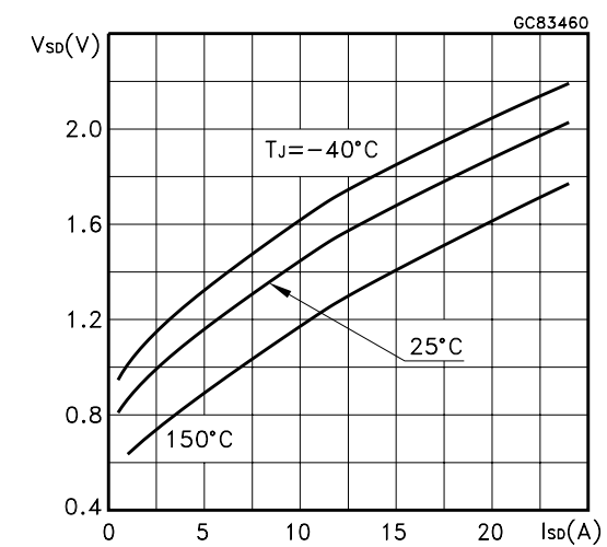
Figure 15: Source-drain Diode Forward Characteristics
